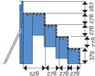
H.1,50m - 4 marches
