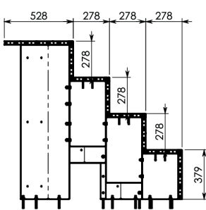
H.1,50m - 4 marches
